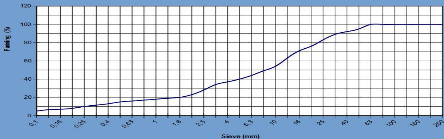
DRAGON 15 Material : Limestone Feeding Size 0 - 1100 mm Rotor Speed : 36 m/sc Adjustment : 40 mm Capacity : 200- 300t/h
